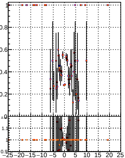
Fake rate vs d D0M D0S MS del8 del9 del10 del11 del12 D0M D0S MS del8 del9 del10 del11 del12
