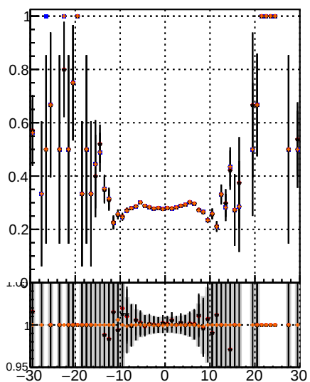
Fake rate vs d D0M D0S MS del8 del9 del10 del11 del12 D0M D0S MS del8 del9 del10 del11 del12
