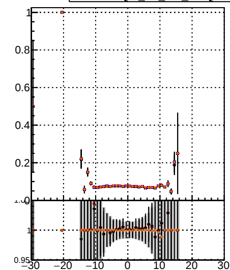
Fake rate vs v BQM TT MS det0 BQM TT MS det0-dpdq BQM TT MS det0-chiz BQM TT MS det0-chiz-dpdq
