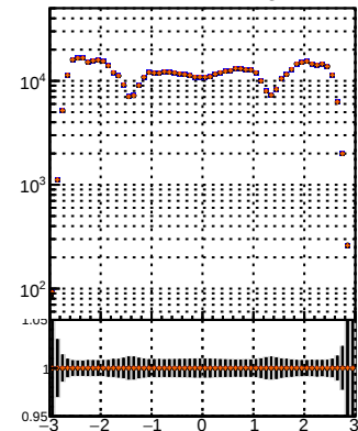
N of reco track vs \eta Legend: BQM TT MS detQ-dm2d
