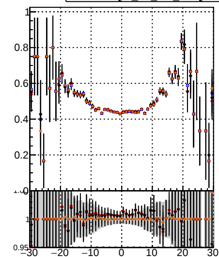
Fake rate vs v Legend: DOM TT MS det0-dpdq (blue squares), DOM TT MS det0-chiz (red circles), DOM TT MS det0 (green triangles), DOM TT MS (orange diamonds)
