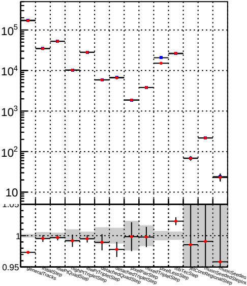
Number of tracks vs collection Legend: Orig/DQM_orig_MS (blue line), pixelLessOrig/DQM_mod_MS (red line)
