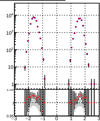
\eta [rad]
