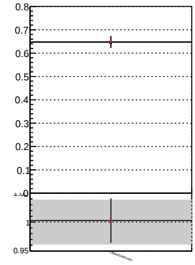
Fake rate vs. — Orig/DQM_orig_MS — pixelLessOrig/DQM_mod_MS
