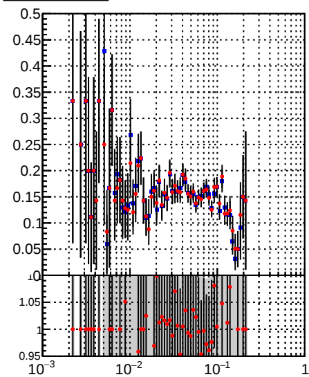
Fake rate vs dr Duplicates Rate vs dr Pileup rate vs dr
