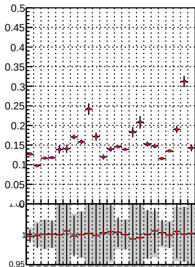
Fake rate vs. Orig/DQM_orig_MS pixelLessOrig/DQM_mod_MS
