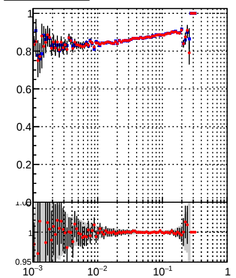
Legend: Orig/DQM_orig_MS (blue line with markers), pixellLessOrig/DQM_mod_MS (red line with markers)
