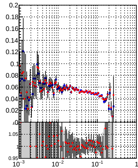
Legend: Orig/DQM_orig_MS (blue line with markers), pixellLessOrig/DQM_mod_MS (red line with markers)
