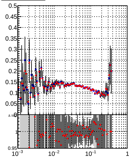
Fake rate vs dr Legend: Orig/DQM_orig_MS pixellLessOrig/DQM_mod_MS
