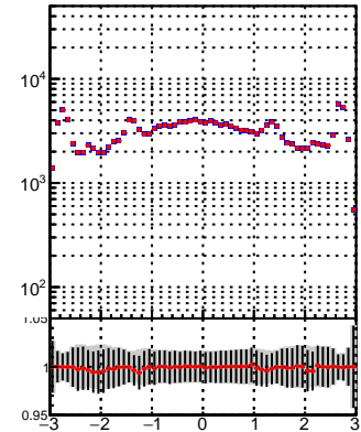
N of reco track vs \eta pixelLessOrig/DQM_mod_MS
