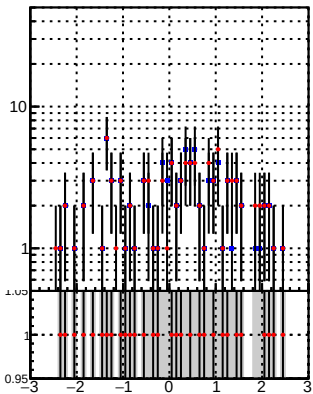
N of reco track vs \eta Orig/DQM_orig_MS pixelLessOrig/DQM_mod_MS
