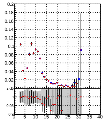
Legend: Orig/DQM_orig_MS (blue line with markers), pixelLessOrig/DQM_mod_MS (red line with markers)
