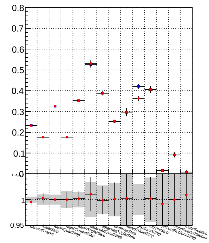
Duplicates rate vs collection Legend: Orig/DQM_orig_MS (blue square) pixelLessOrig/DQM_mod_MS (red circle)
