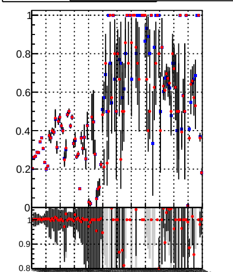
Fake rate vs. —●— Orig/DQM_orig_MS —●— pixelLessOrig/DQM_mod_MS
