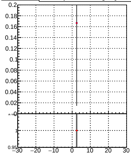
Fake rate vs vertpos Orig/DQM_orig_MS pixellLessOrig/DQM_mod_MS
