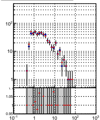
N of reco track vs pT pixelLessOrig/DQM_mod_MS
