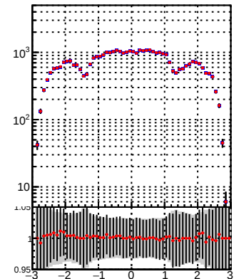
N of reco track vs \eta Orig/DQM_orig_MS pixelLessOrig/DQM_mod_MS
