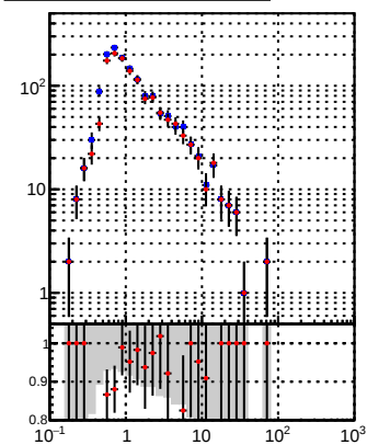
N of reco track vs \eta pixelLessOrig/DQM_mod_MS
