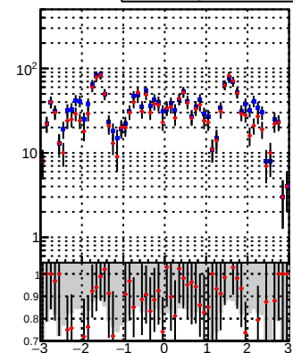
N of reco track vs \eta pixelLessOrig/DQM_mod_MS
