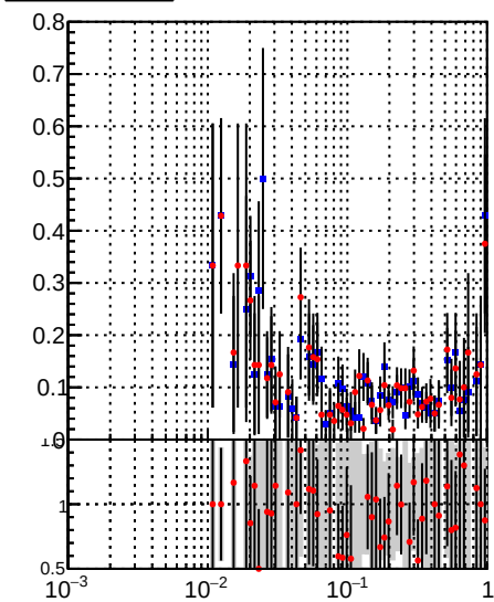
Legend: Orig/DQM_orig_MS (blue squares), pixellLessOrig/DQM_mod_MS (red circles)
