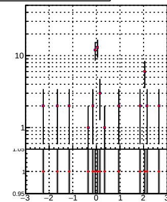
N of associated (recoToSim) tracks vs \eta Orig/DQM_orig_MS pixelLessOrig/DQM_mod_MS
