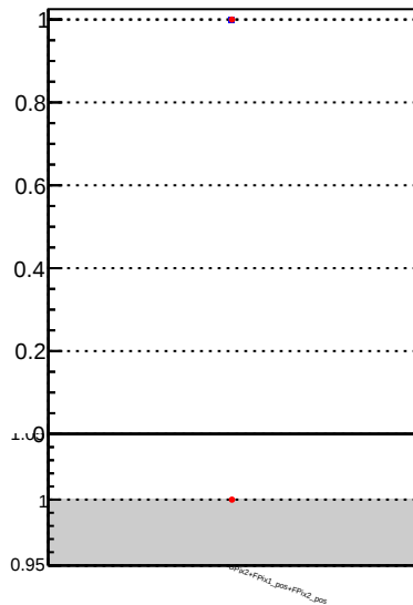
Fake rate vs. —•— Orig/DQM_orig_MS —•— pixelLessOrig/DQM_mod_MS
