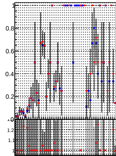
Fake rate vs. —•— Orig/DQM_orig_MS —•— pixelLessOrig/DQM_mod_MS
