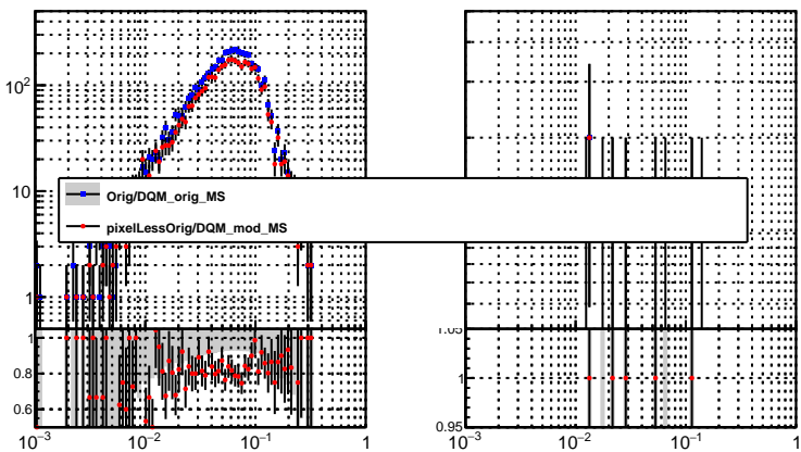
N of associated (recoToSim) looped tracks vs dR
