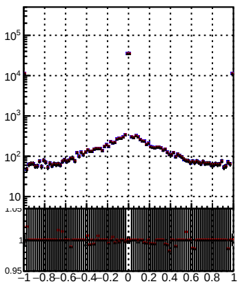
N of sim \longrightarrow pixelLess/DQM_mod_MS
