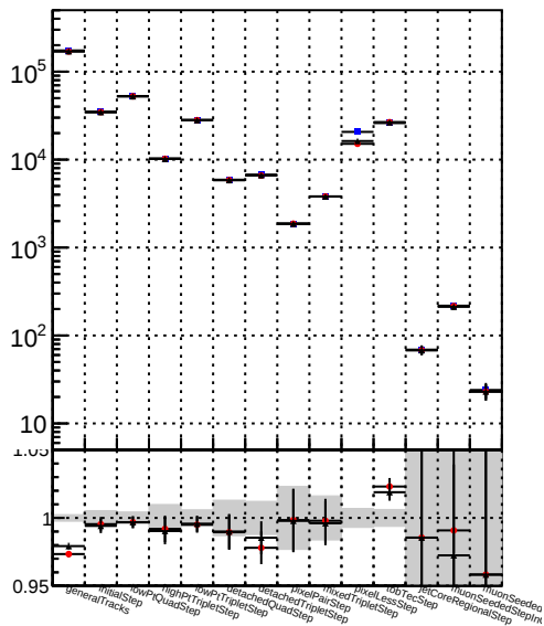
Number of tracks vs collection Legend: Orig/DQM_orig_MS (blue line with dots) pixelLessOrig/DQM_mod_MS (red line with dots) pixelLess/DQM_mod_MS (black line with dots)
