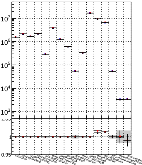
Number of tracks vs collection Legend: Orig/DQM_orig_MS (blue line) pixelLessOrig/DQM_mod_MS (red line) pixelLess/DQM_mod_MS (black line)
