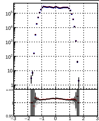
N of reco track vs \eta —●— Orig/DQM_orig MS —●— pixelLess/DQM_orig MS —●— pixelLess/DQM_mod MS
