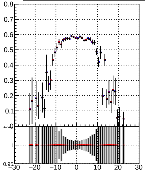
Efficiency vs. sim PV z Legend: Orig/DQM_orig_MS (blue line with dots) pixelLessOrig/DQM_mod_MS (red line with dots) pixelLess/DQM_mod_MS (black line with dots)
