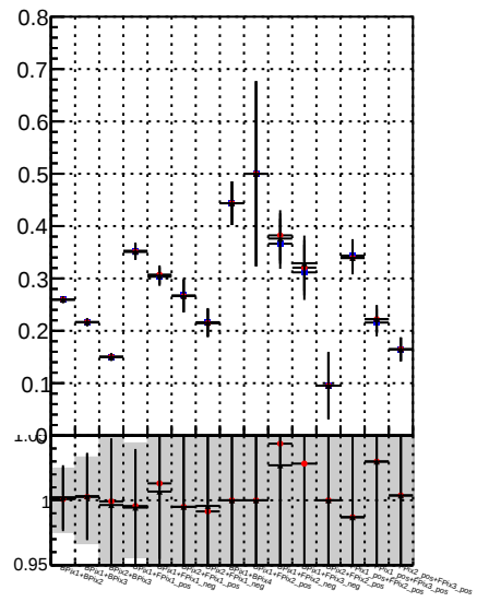
Fake rate vs. — Orig/DQM_orig_MS — pixelLess/DQM_orig_MS — pixelLess/DQM_mod_MS
