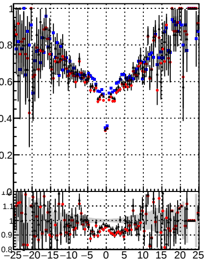
Fake rate vs d — Orig/DQM_orig_MS — PixelLess/DQM_mod_MS
