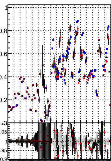
Fake rate vs. —●— Orig/DQM_orig_MS —●— pixelLess/DQM_orig_MS —●— pixelLess/DQM_mod_MS
