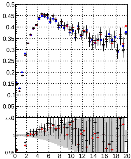
Fake rate vs. —●— Orig/DQM_orig_MS —●— pixelLess/DQM_orig_MS —●— pixelLess/DQM_mod_MS
