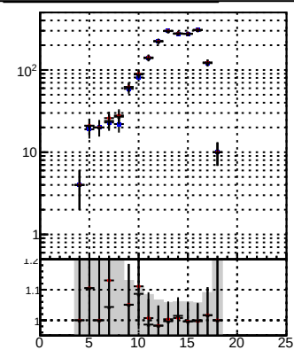
N of reco track vs hit Orig/DQM orig MS pixelLess/DQM mod MS pixelLess/DQM mod MS
