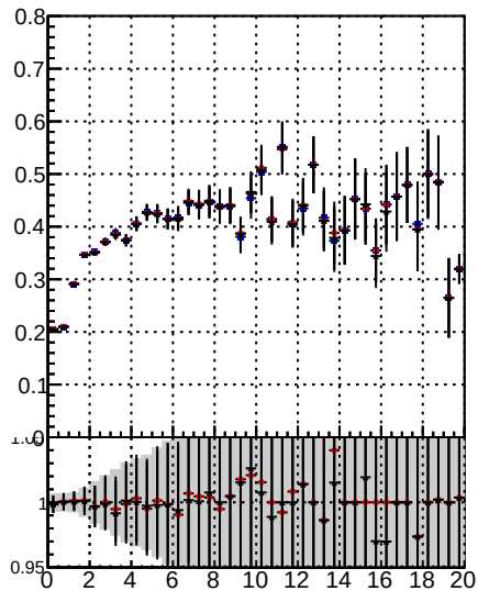
Fake rate vs. — Orig/DQM_orig_MS — pixelLess/DQM_mod_MS — pixelLess/DQM_mod_MS
