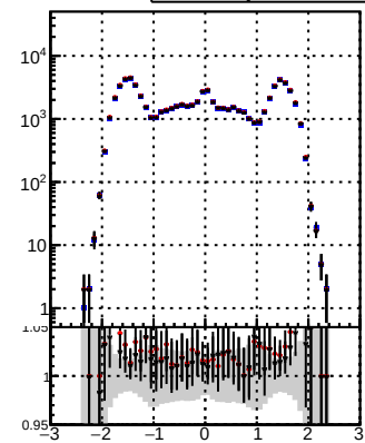
N of reco track vs \eta Orig/DQM MS pixelLess/DQM mdd MS pixelLess/DQM mod MS
