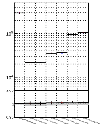
N of reco track vs. \chi^2 — pixelLessOrig/DOM_mod MS — pixelLessOrig/DOM_mod MS — pixelLessOrig/DOM_mod MS
