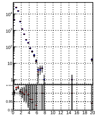
N of reco (recoToSim) tracks vs normalized \chi^2
