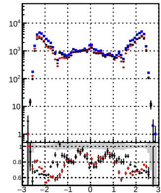
N of reco track vs \eta —●— pixelLess/DQM orig MS —●— pixelLess/DQM orig MS —●— pixelLess/DQM mod MS —●— pixelLess/DQM mod MS
