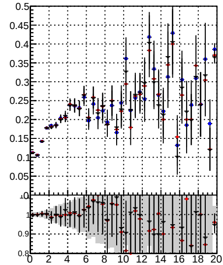
Fake rate vs. — Orig/DQM_orig_MS — Less/DQM_orig_MS — Less/DQM_mod_MS
