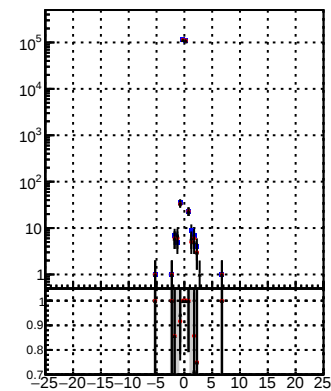
N of reco track vs dxy(PV) Legend: Orig/DQM orig MS (blue line with dots) pixelLessOrig/DQM mod MS (red line with dots) pixelLess/DQM mod MS (black line with dots)
