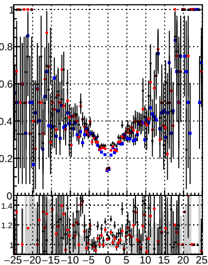
Fake rate vs d —●— Orig/DQM_orig_MS —●— PixelLess/DQM_orig_MS —●— PixelLess/DQM_mod_MS
