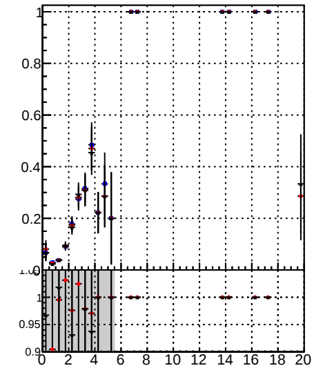
Fake rate vs. —●— Orig/DQM_orig_MS —●— pixelLess/DQM_orig_MS —●— pixelLess/DQM_mod_MS
