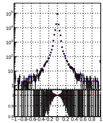
N of reco track vs dxy(PV) Legend: Orig/DQM orig MS pixelLessOrig/DQM mod MS pixelLess/DQM mod MS
