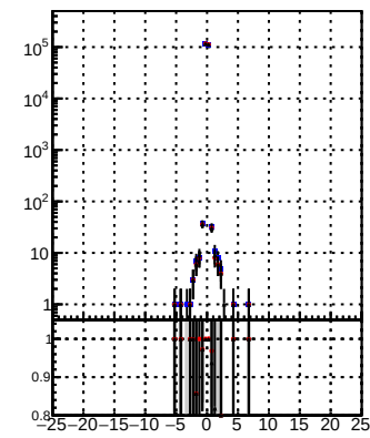
N of reco track vs dxy(PV) Legend: Orig/DQM orig MS pixelLessOrig/DQM mod MS pixelLess/DQM mod MS
