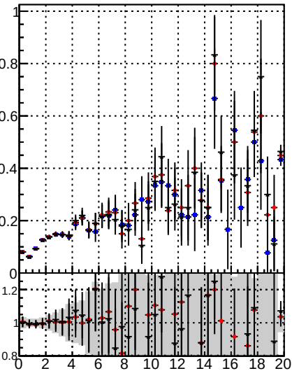
Fake rate vs. — Orig/DQM_orig_MS — pixelLess/DQM_mod_MS — pixelLess/DQM_mod_MS
