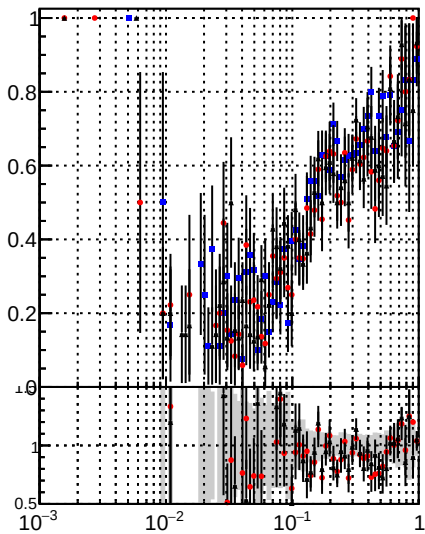
Fake rate vs \sqrt{s} Legend: —●— Orig/DQM orig_MS —●— pixelLessOrig/DQM_mod_MS —●— pixelLess/DQM_mod_MS
