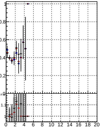
Fake rate vs. Orig/DQM orig MS Less/DQM orig MS Less/DQM mod MS
