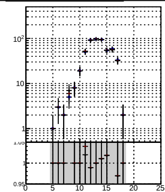
N of reco track vs hit Orig/DQM orig MS pixelLess/DQM mod MS
