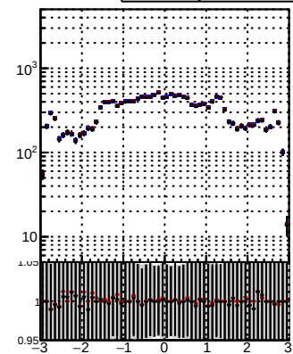
N of reco track vs \eta Orig/DQM orig MS pixelLess/DQM mod MS pixelLess/DQM mod MS
