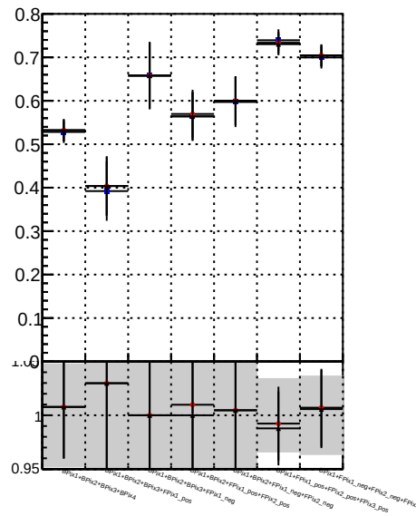
Fake rate vs. — Orig/DQM_orig_MS — pixelLess/DQM_orig_MS — pixelLess/DQM_mod_MS
